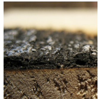
Photo showing the protective charcoal layer
