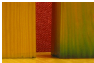
The untreated end grain on the component on the right acts like a blotting paper, sucking in moisture
