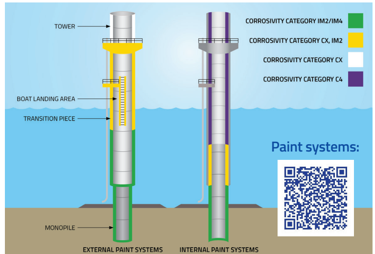
Coatings for buried, submerged, splash and atmospheric zones of internal and external foundation structures according to EN ISO 12944-5 corrosivity categories.
