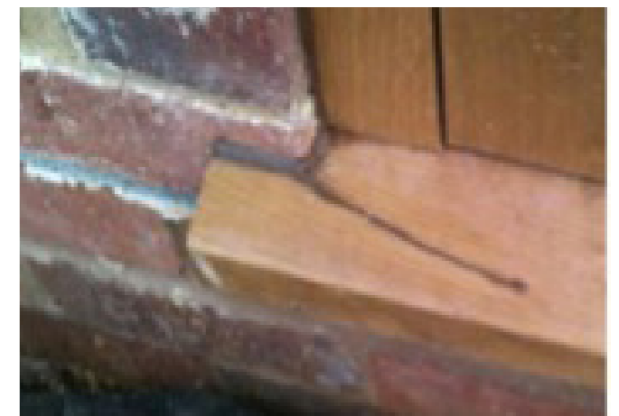
The surface of oak joinery tends to split in service, disrupting the protective coating, allowing water to enter and react with Tannic Acid
